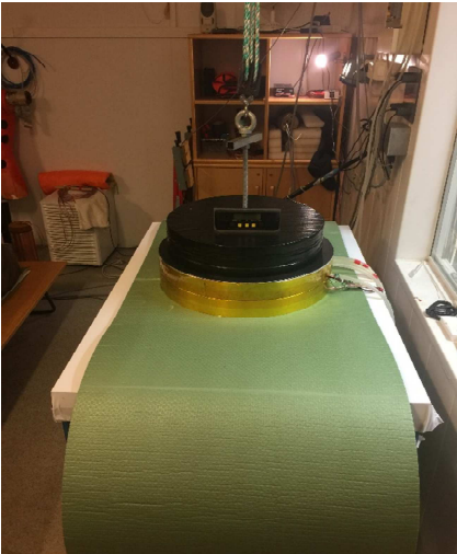
FIG. A3.3 Front View of Testing
